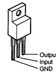
NJM7908FA (IC504)
